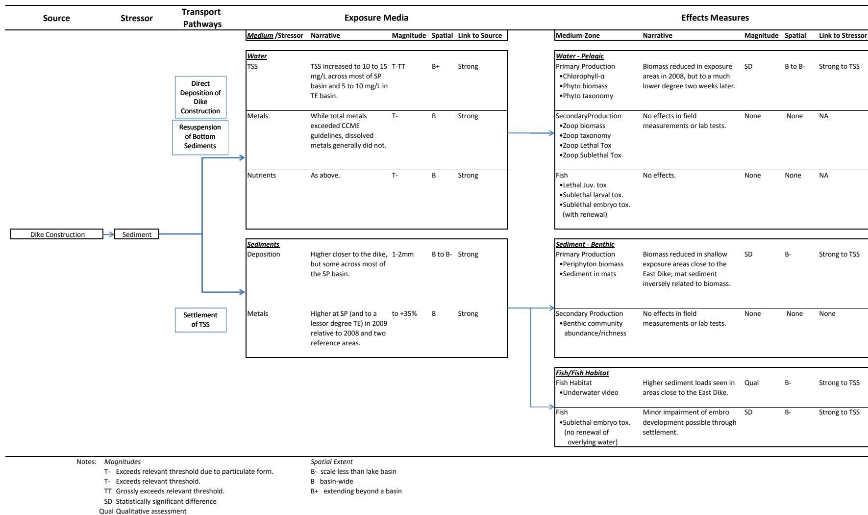
Figure 4-5. Example of an issue-specific conceptual site model for the 2008 sedimentation event during East Dike construction
